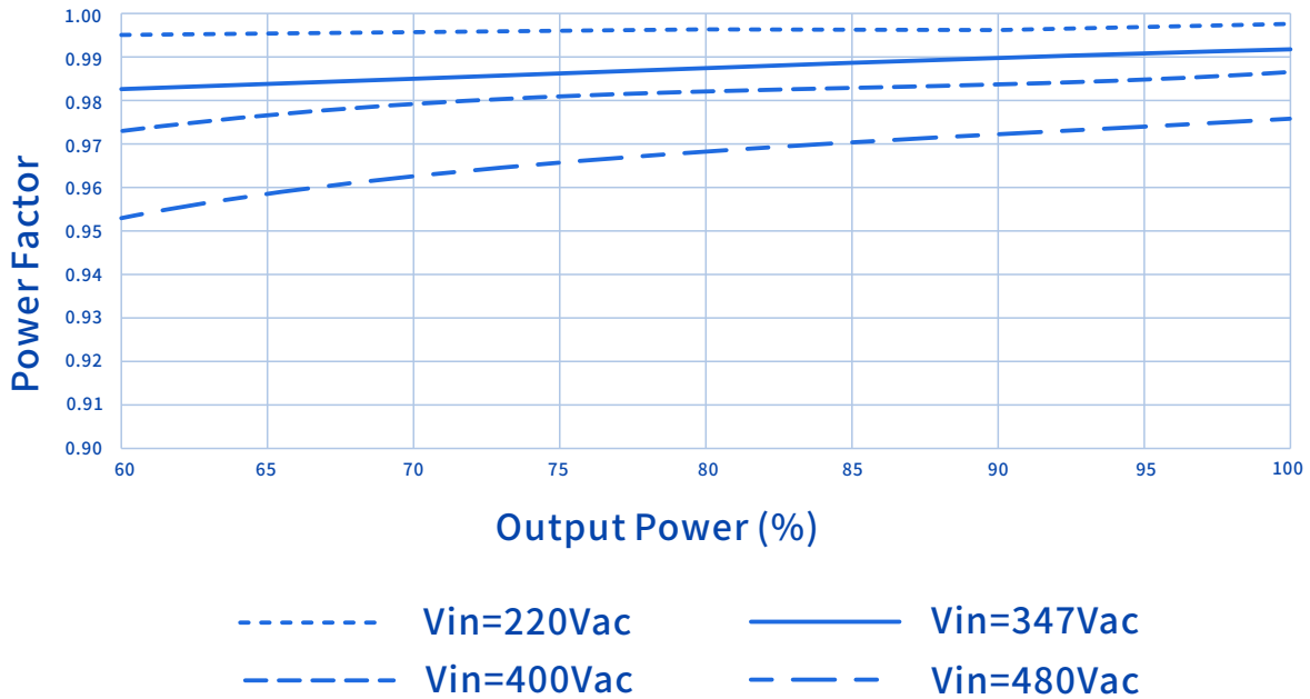
Power Factor Vs. O/P Power
